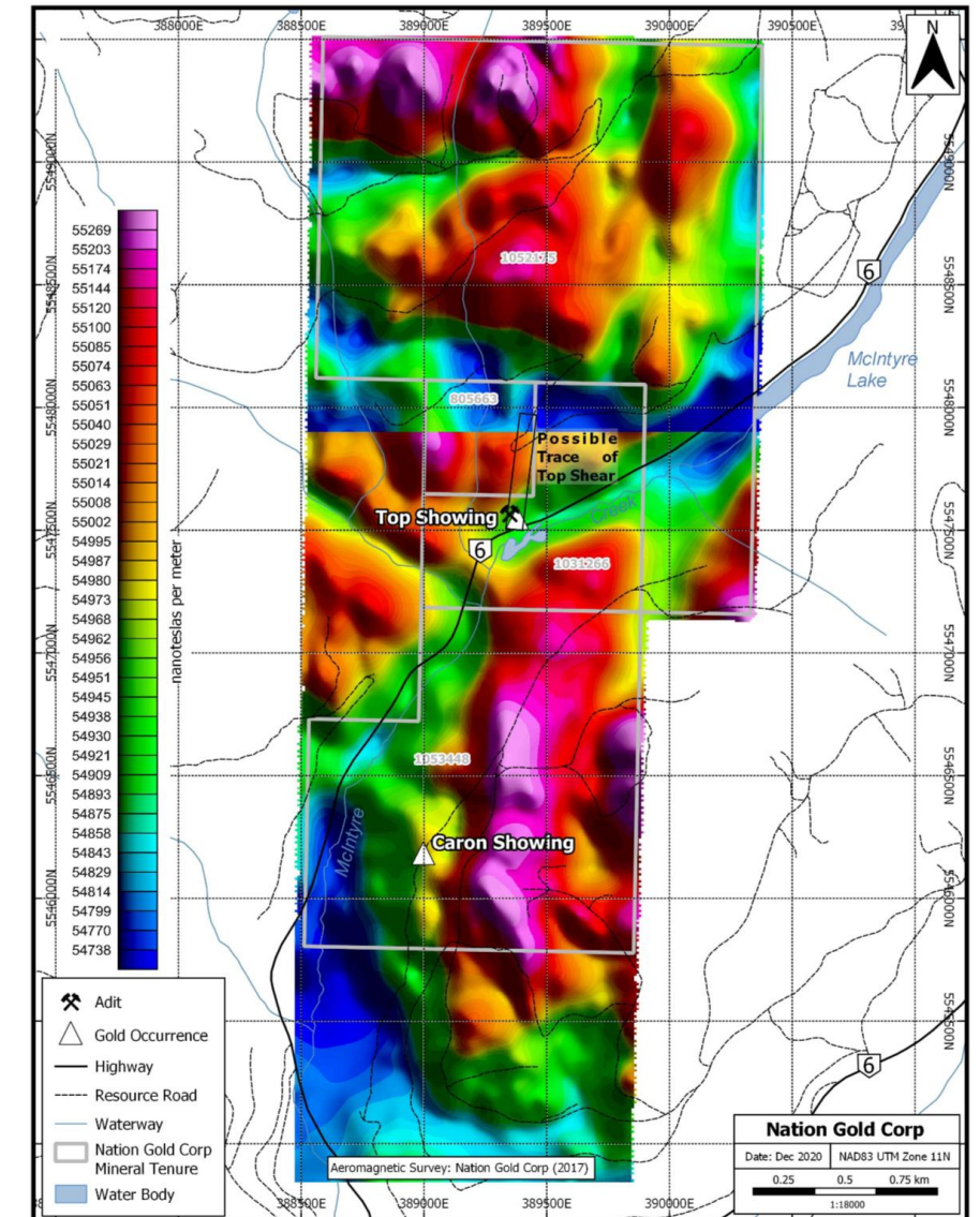
2017 Aeromagnetic Survey - Total Magnetic Intensity Plan
